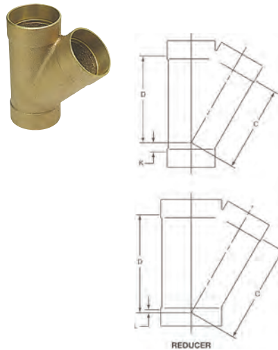
810 ⚠ DWV 45° Y C x C x C – Cast
