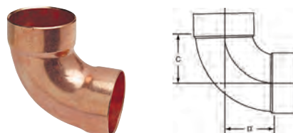
907 DWV 90° Elbow C x C – Wrot
