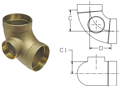
807-9 ⚠ DWV 90° Elbow w/Side Inlet C x C x C – Cast
