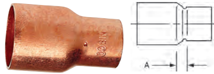
600 Reducing Coupling C x C – Wrot
