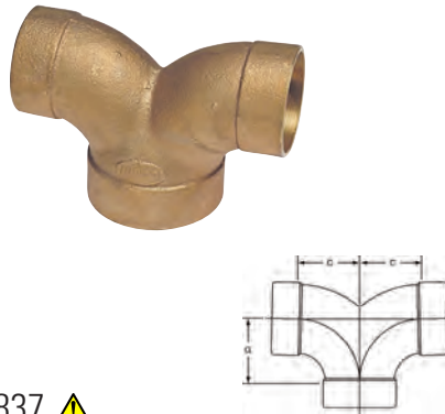
837 ⚠ DWV 90° Double Elbow C x C x C – Cast
