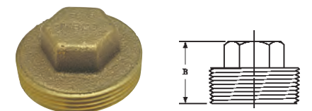
818 A.S.A. ⚠ DWV Plug M – Cast
