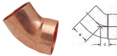
906-2 DWV 45° Fitting Elbow Ftg x C – Wrot
