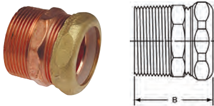
904-7 DWV Trap Adapter M x SJ – Wrot
