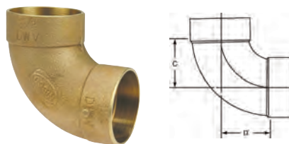
807 ⚠ DWV 90° Elbow C x C – Cast
