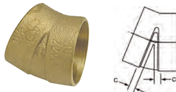
808 ⚠ DWV 22 1 / 2 ° Elbow C x C – Cast
