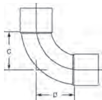
607-1 90° Elbow – Intermediate Radius C x C – Wrot
