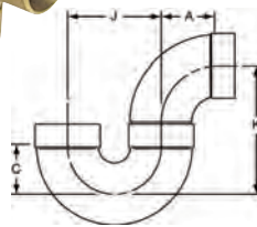
885 ⚠ DWV P-Trap C x C – Cast
