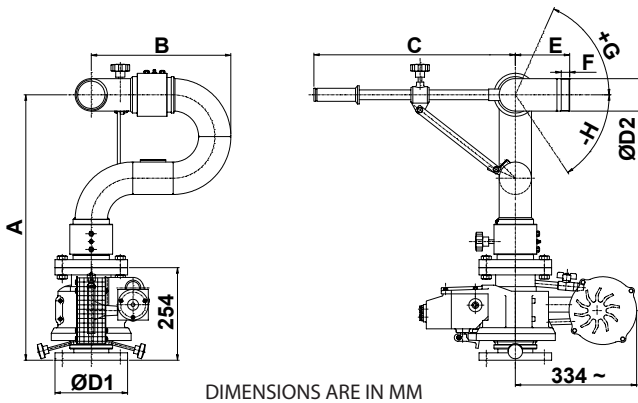
Shown with optional polished stainless steel finish and foam/water branch pipe
